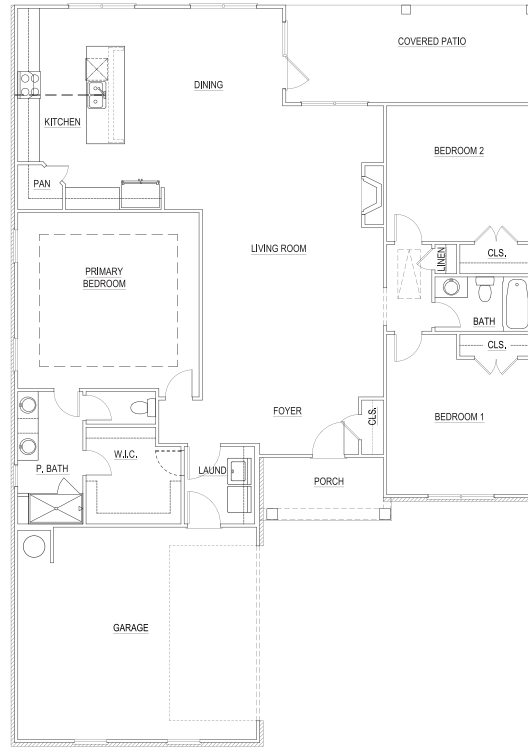
1ST FLOOR PLAN -A-
