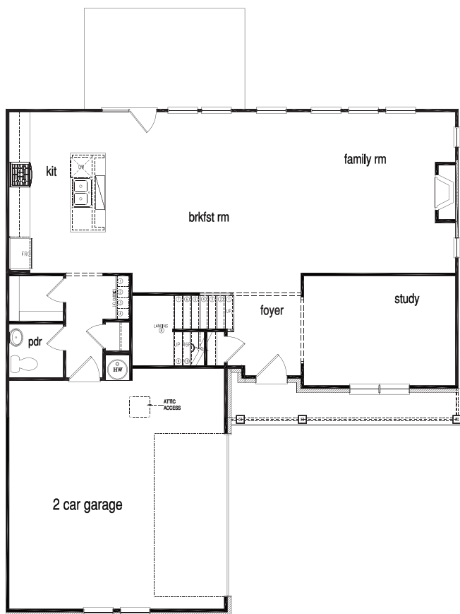
1st Floor Plan 'C'
