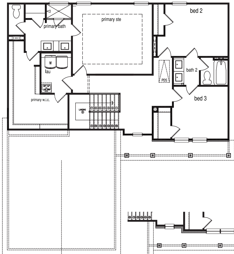
2nd Floor Plan 'A'
