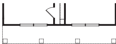
2nd Floor Plan 'B'
