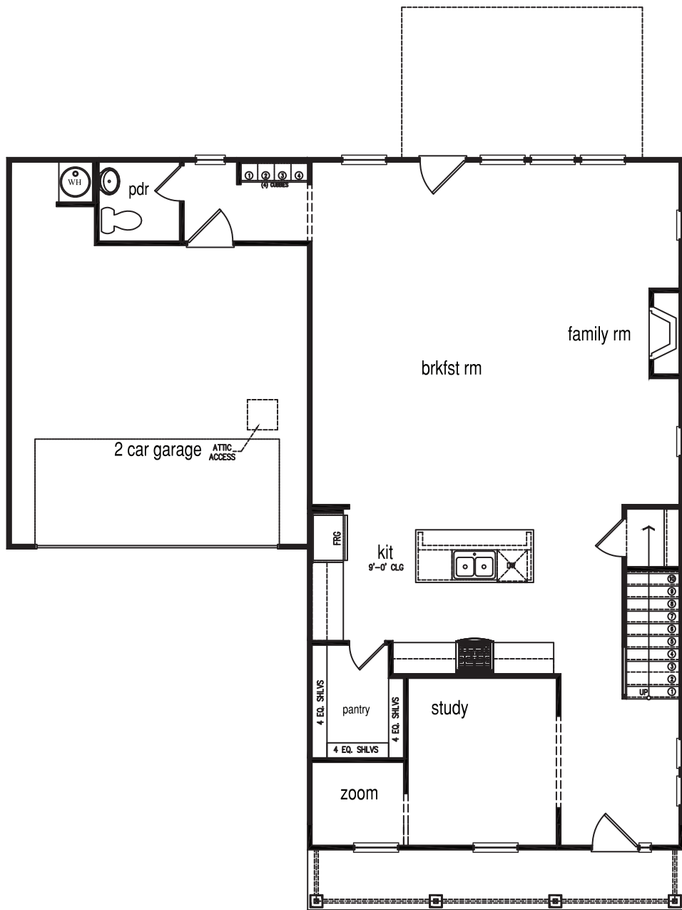
1st Floor Plan 'A'
