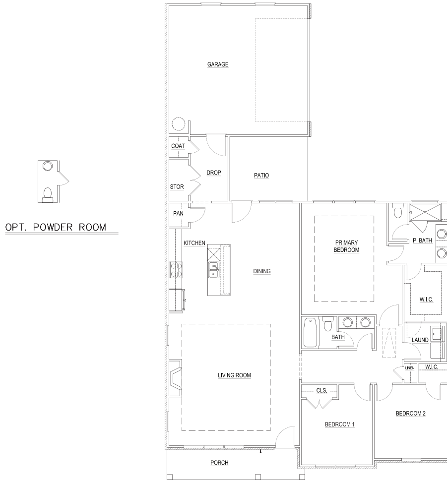
1ST. FLOOR PLAN -A-
