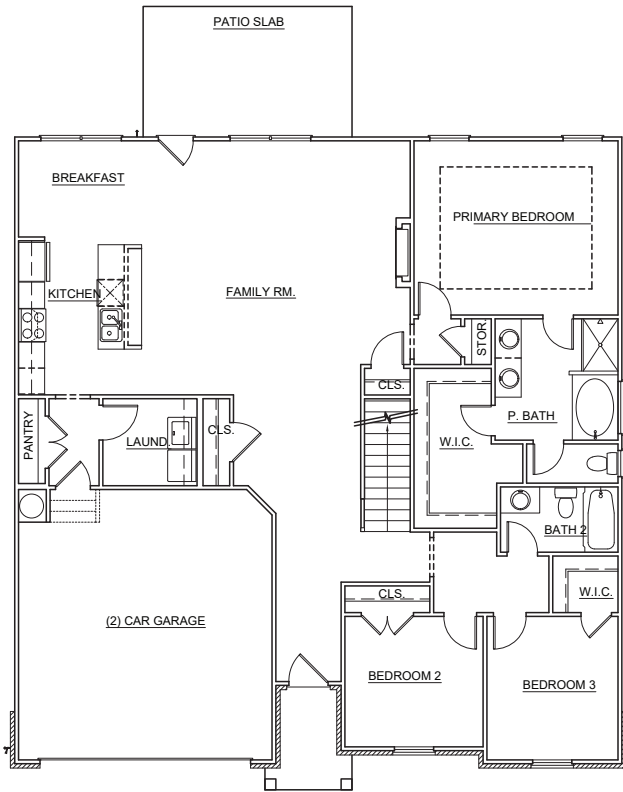
FIRST FLR. PLAN
