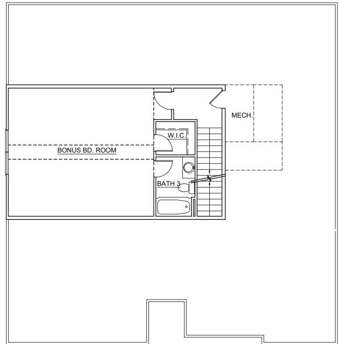
SECOND FLR. PLAN
