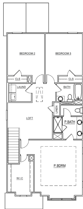
SECOND FLOOR (B) SCALE: 1/8"=1'-0"
