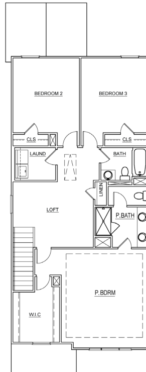
SECOND FLOOR (A) SCALE: 1/8" = 1'-0"
