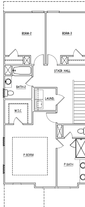
SECOND FLOOR PLAN UNIT - B
