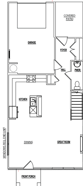
FIRST FLOOR PLAN UNIT - A
