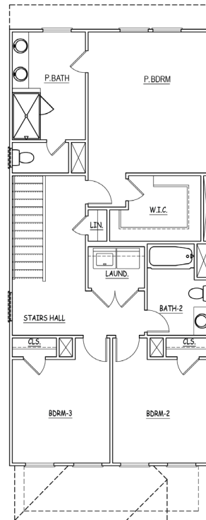
SECOND FLOOR PLAN UNIT - D
