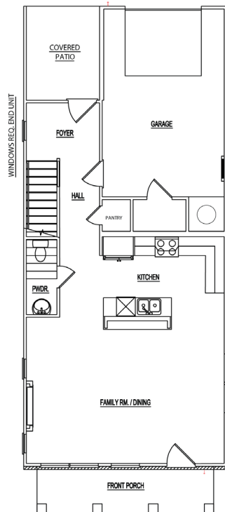
FIRST FLOOR PLAN UNIT - A
