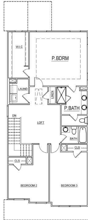
SECOND FLOOR (B) SCALE: 1/8" = 1'-0"
