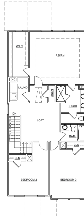
SECOND FLOOR (A) SCALE: 1/4" = 1'-0"
