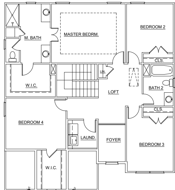
SECOND FLOOR PLAN SCALE : 1/4" = 1'-0"
